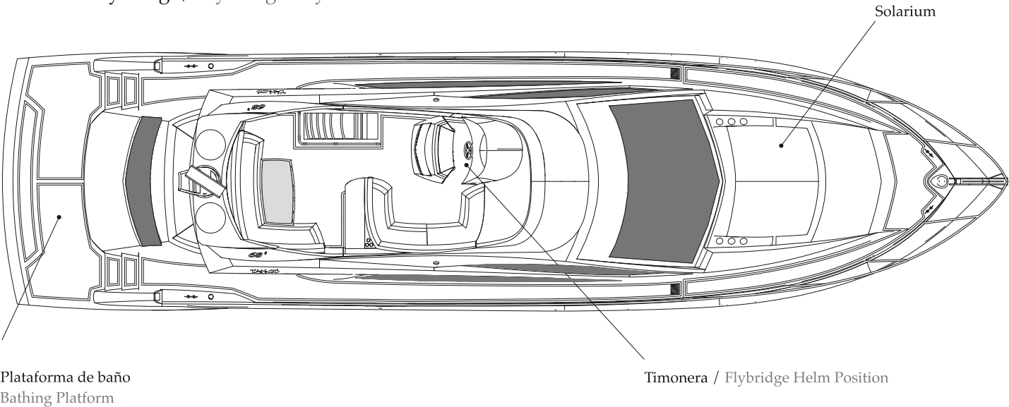
Planta de Flybridge/ Flybridge Layout
